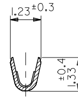
SECT. A-A
